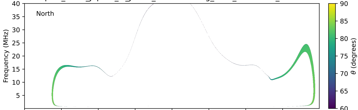
expres_earth_jupiter_io_jrm33_lossc-wid1deg_3kev_20250716_v11.cdf
