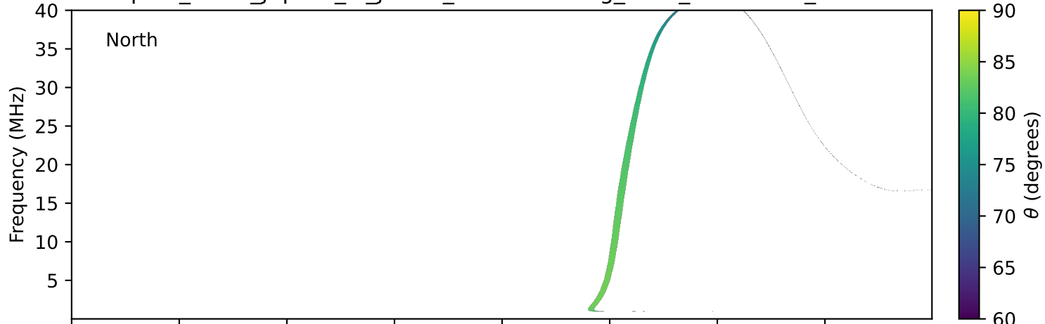
expres_earth_jupiter_io_jrm33_lossc-wid1deg_3kev_20250712_v11.cdf
