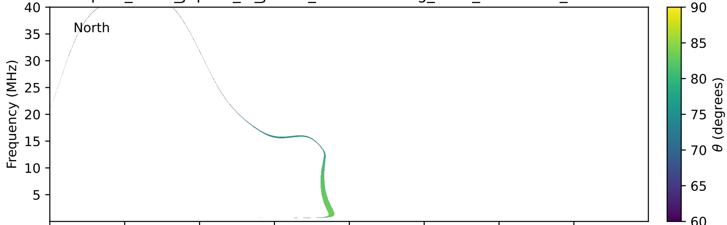
expres_earth_jupiter_io_jrm33_lossc-wid1deg_3kev_20250711_v11.cdf
