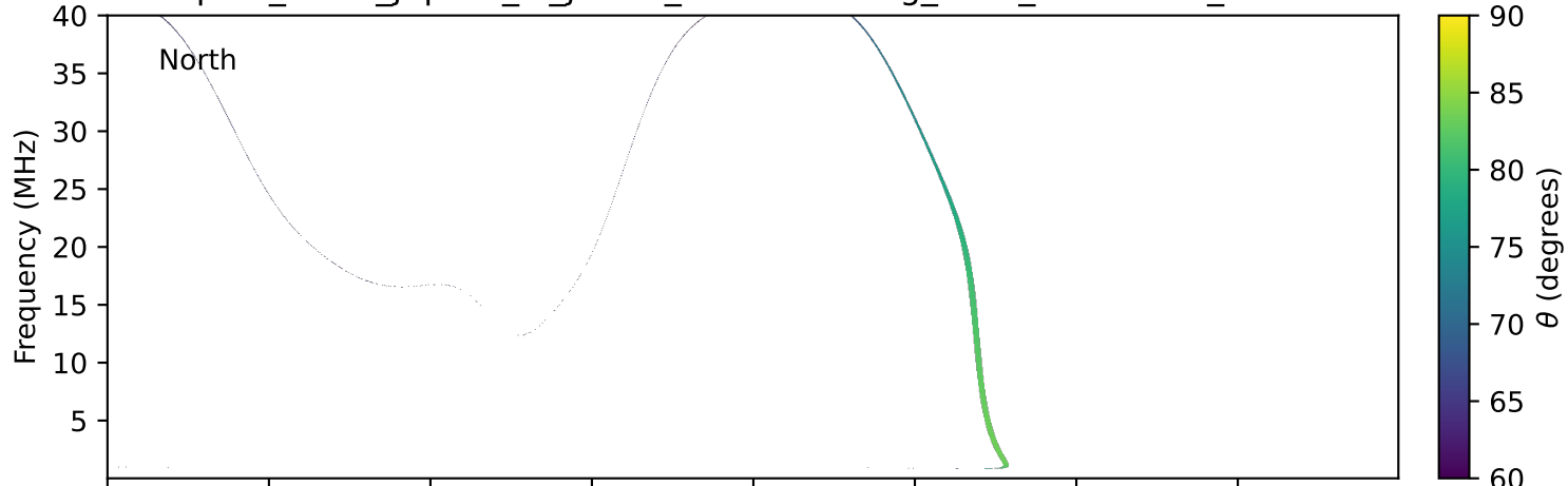
expres_earth_jupiter_io_jrm33_lossc-wid1deg_3kev_20250709_v11.cdf
