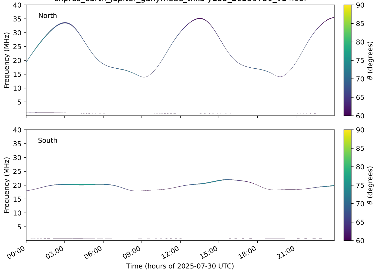
expres_earth_jupiter_ganymede_txka-y235_20250730_v14.cdf
