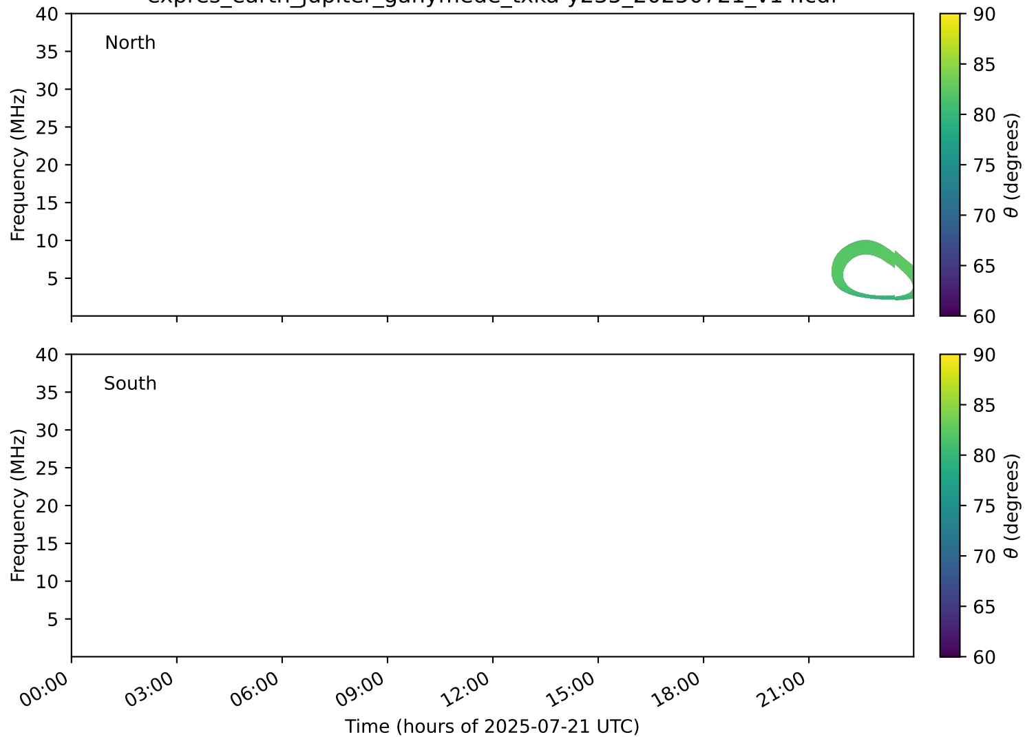
expres_earth_jupiter_ganymede_txka-y235_20250721_v14.cdf
