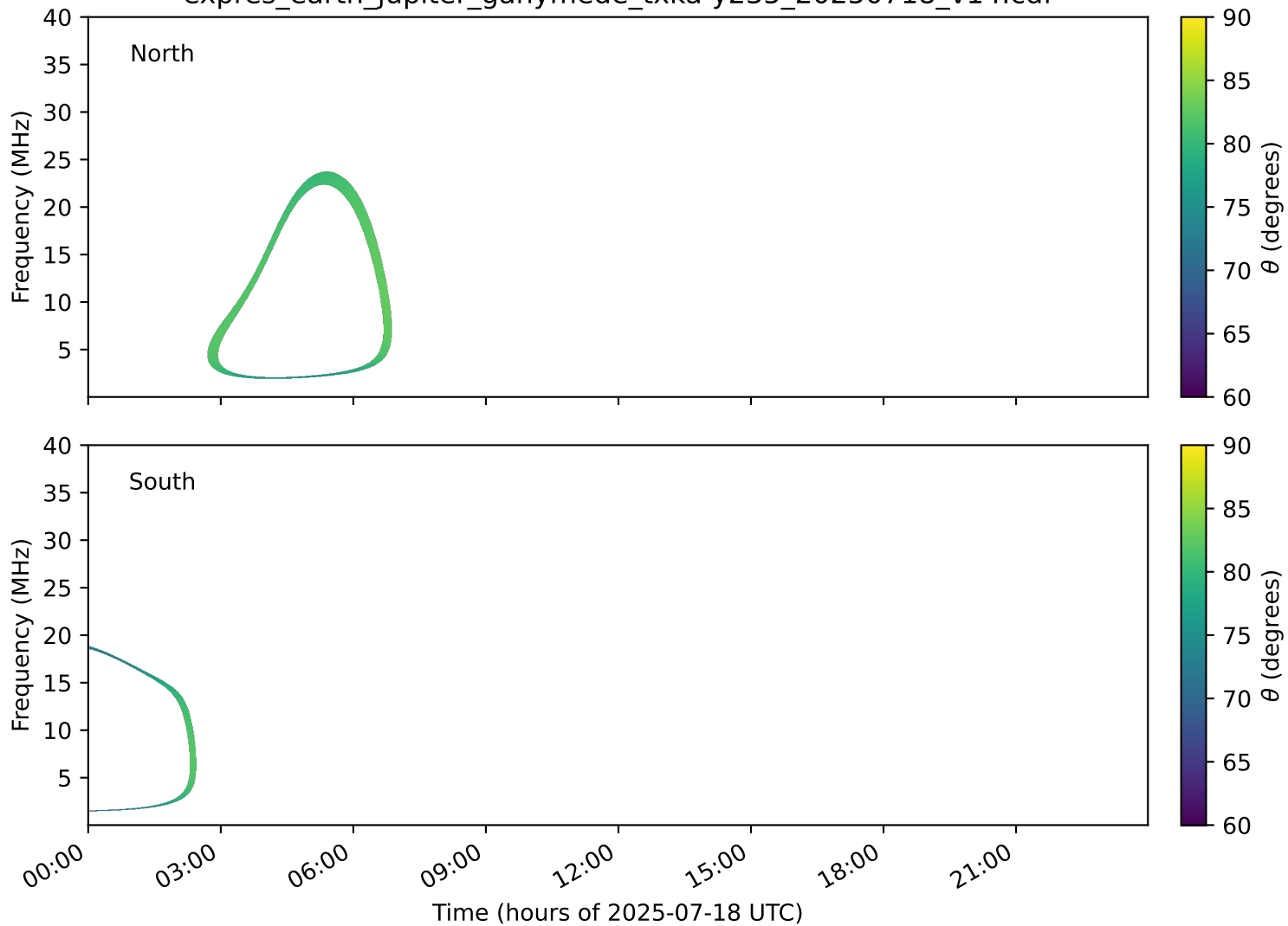
expres_earth_jupiter_ganymede_txka-y235_20250718_v14.cdf
