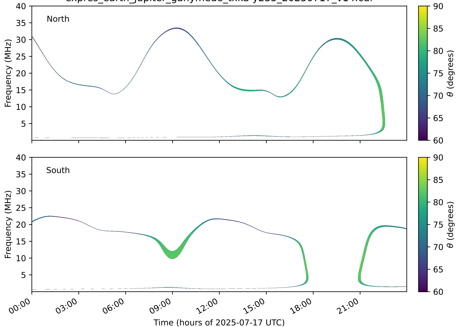
expres_earth_jupiter_ganymede_txka-y235_20250717_v14.cdf
