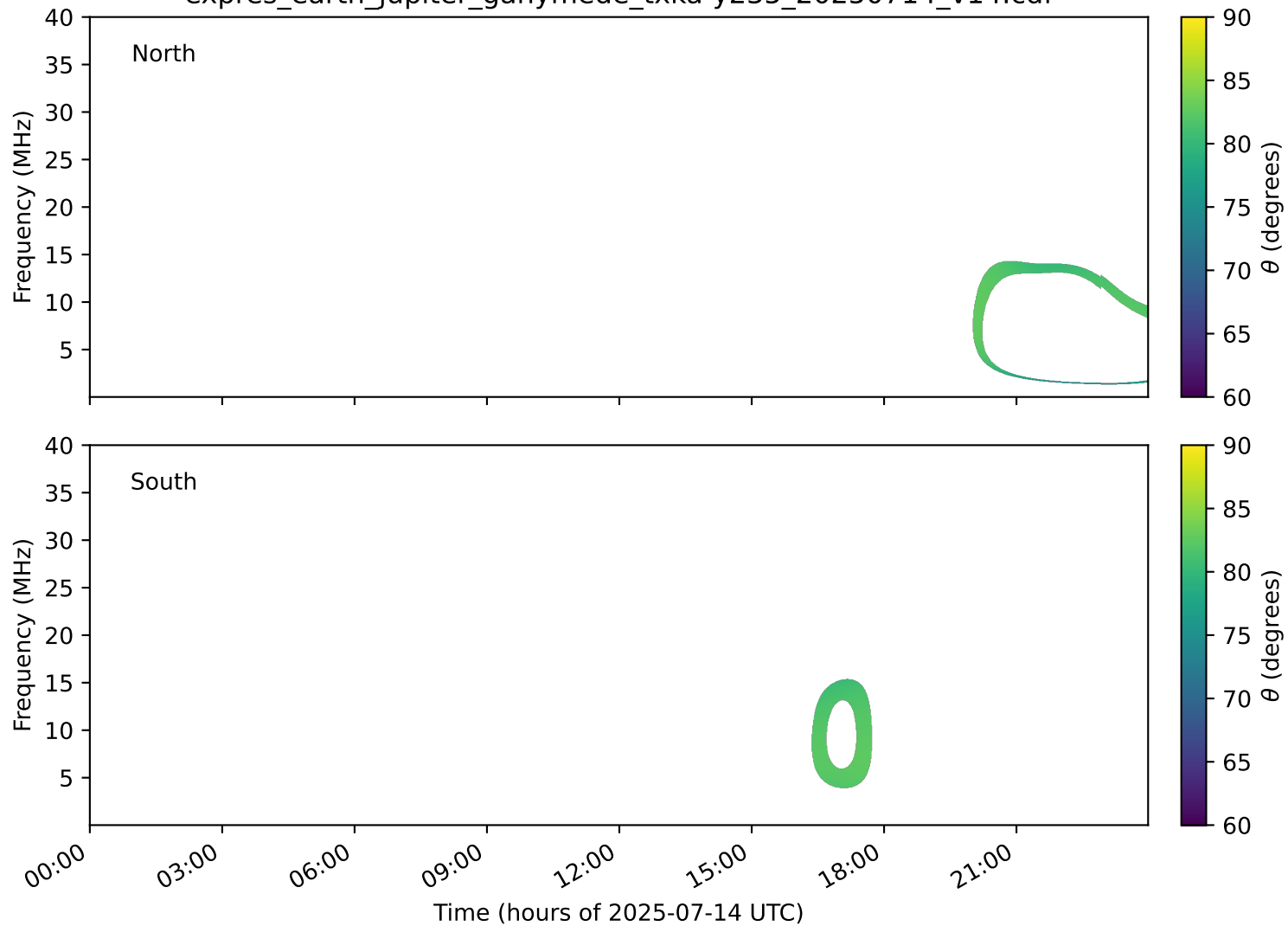
expres_earth_jupiter_ganymede_txka-y235_20250714_v14.cdf
