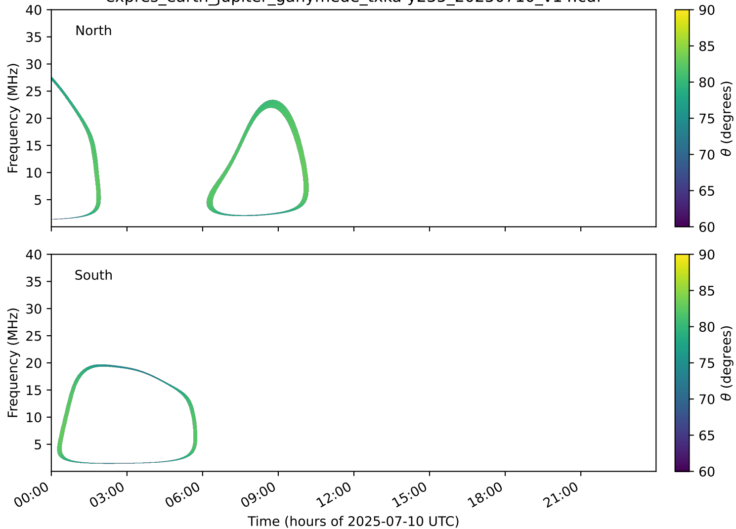
expres_earth_jupiter_ganymede_txka-y235_20250710_v14.cdf
