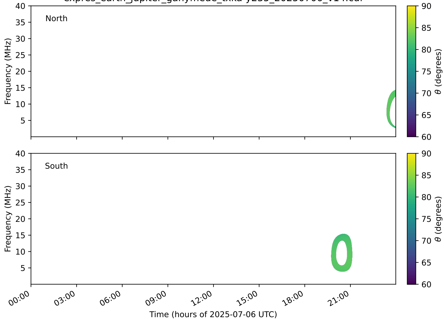
expres_earth_jupiter_ganymede_txka-y235_20250706_v14.cdf
