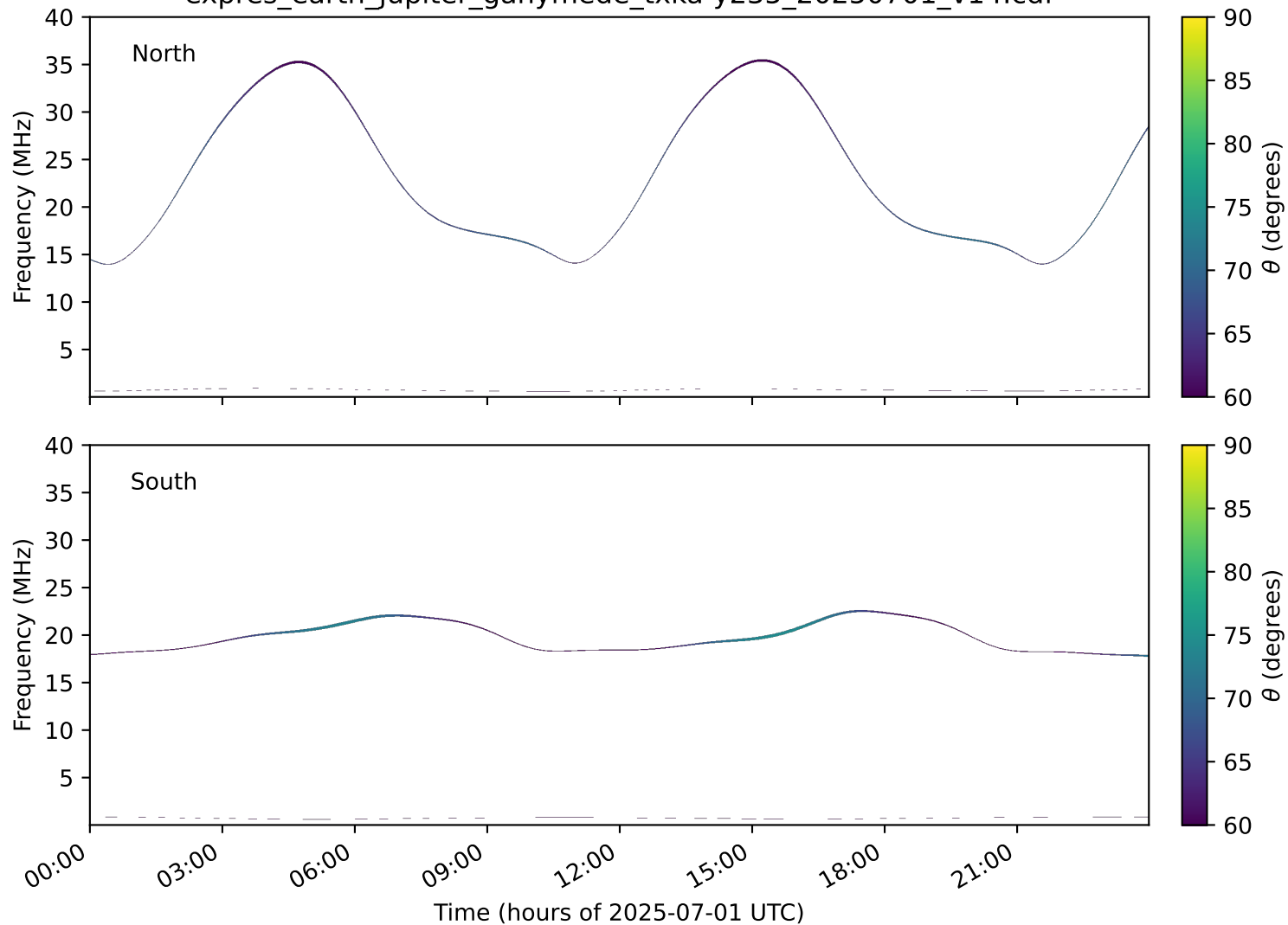
expres_earth_jupiter_ganymede_txka-y235_20250701_v14.cdf
