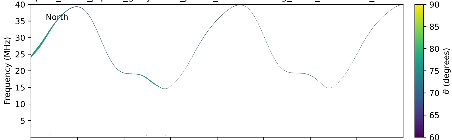
expres_earth_jupiter_ganymede_jrm33_lossc-wid1deg_3kev_20250730_v11.cdf
