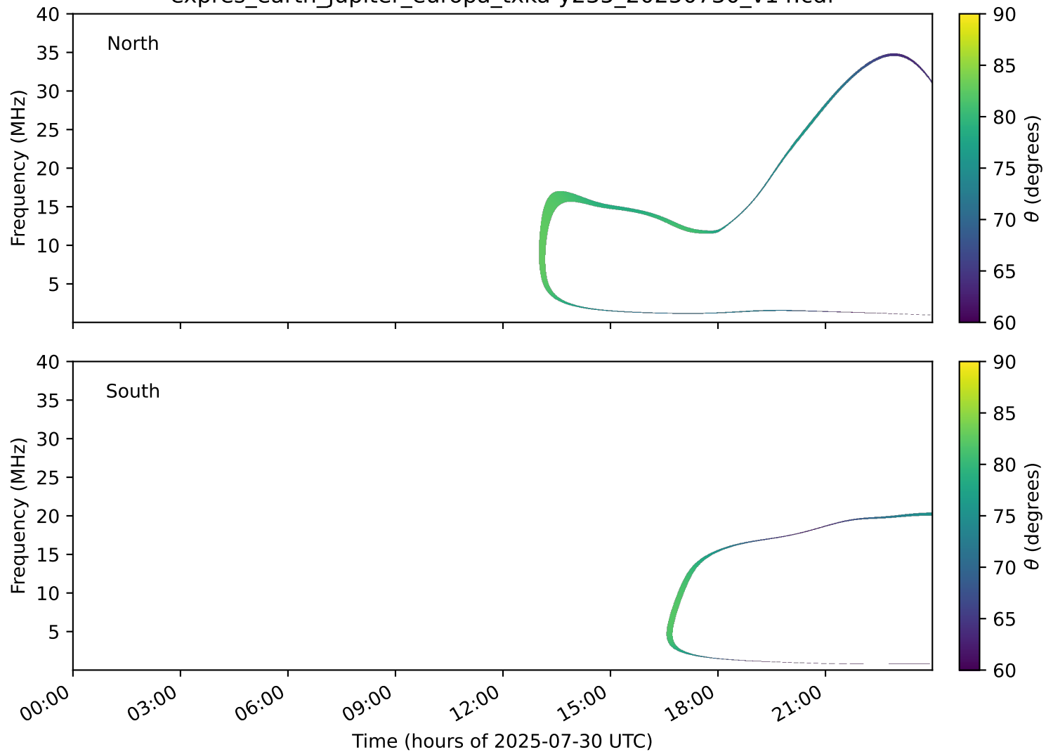
expres_earth_jupiter_europa_txka-y235_20250730_v14.cdf
