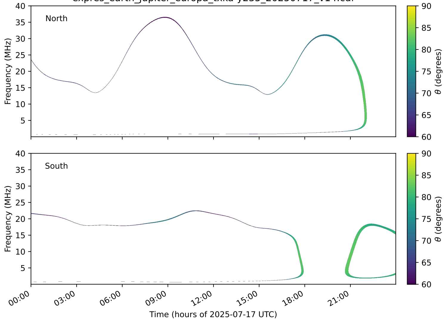
expres_earth_jupiter_europa_txka-y235_20250717_v14.cdf
