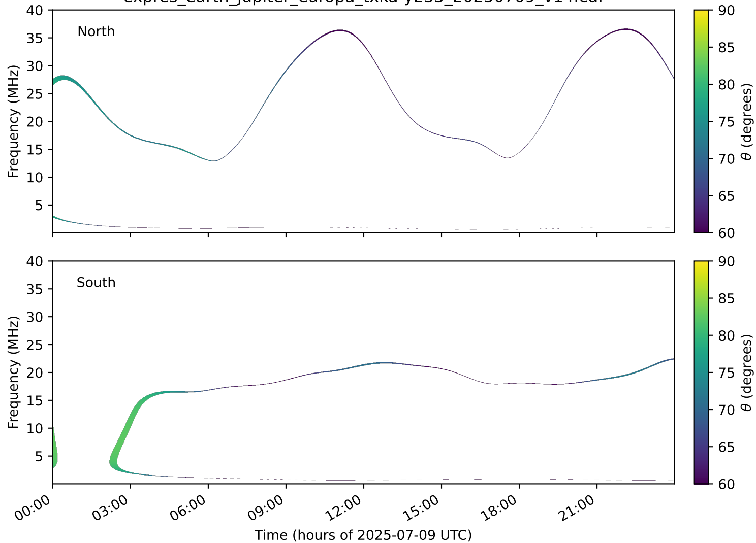
expres_earth_jupiter_europa_txka-y235_20250709_v14.cdf
