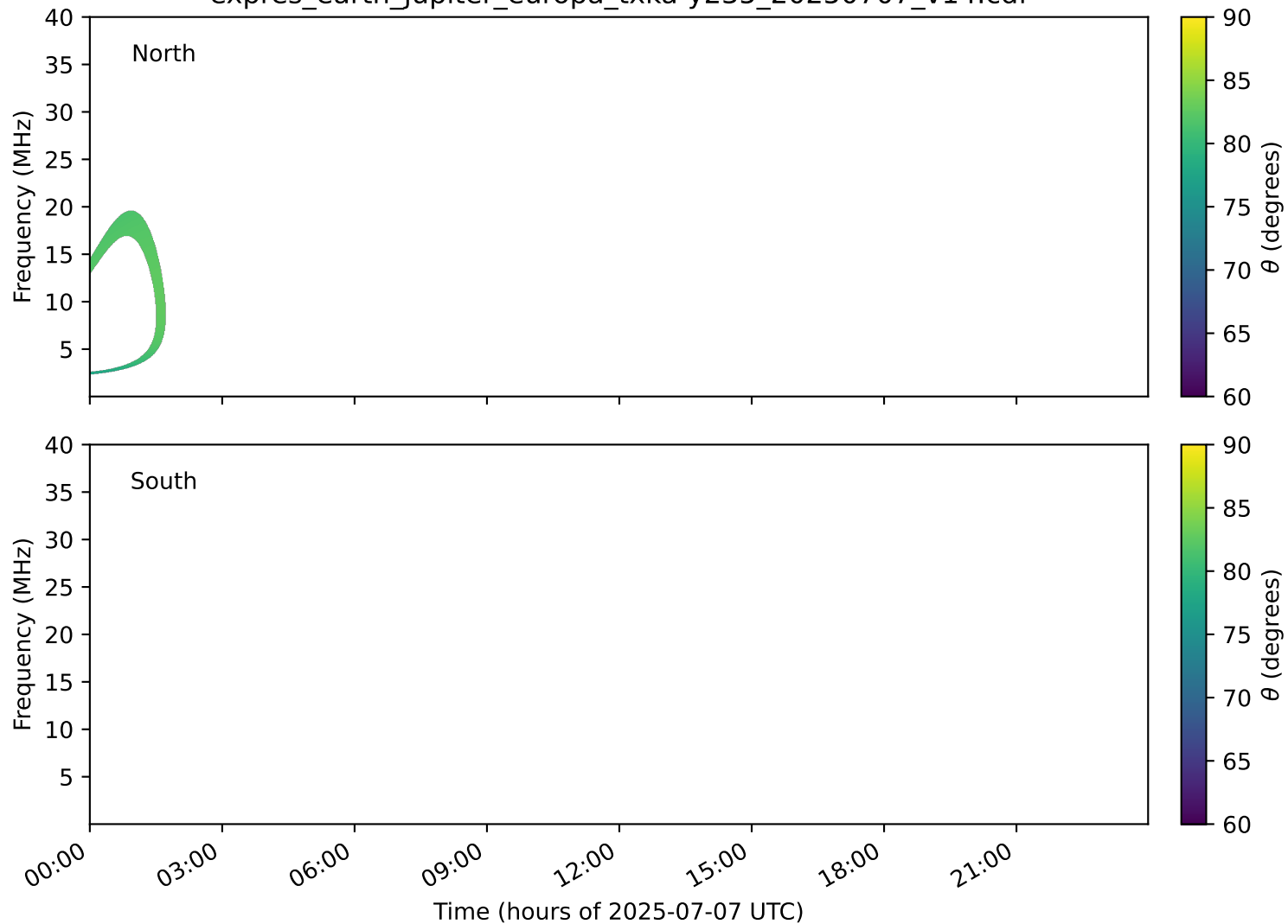
expres_earth_jupiter_europa_txka-y235_20250707_v14.cdf
