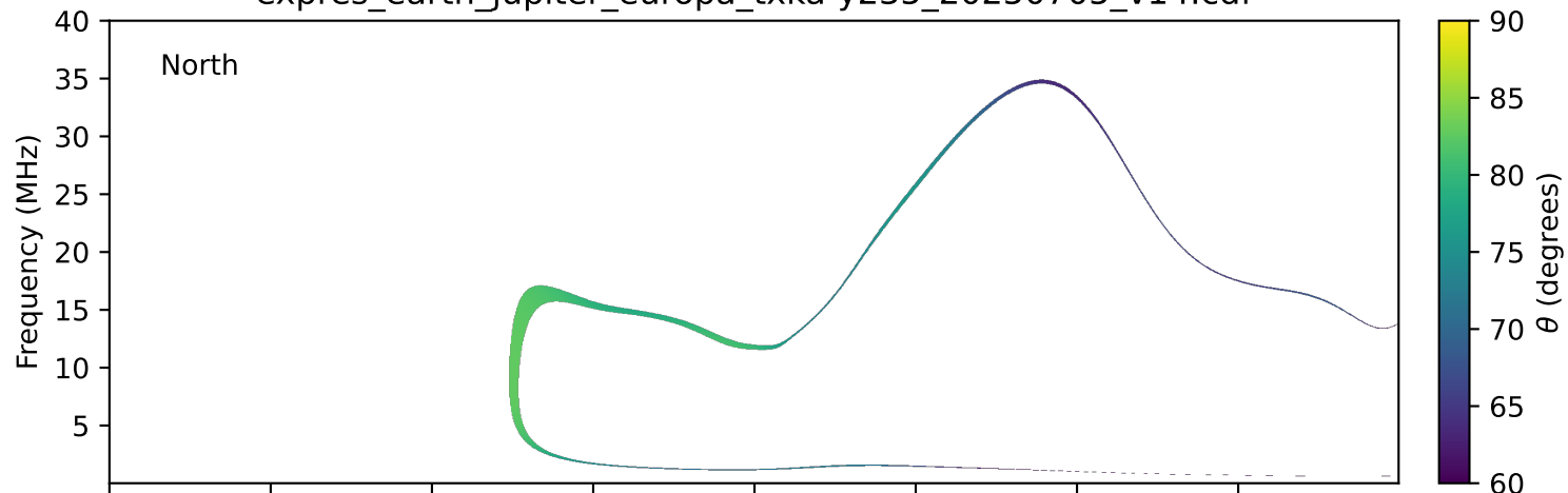
expres_earth_jupiter_europa_txka-y235_20250705_v14.cdf
