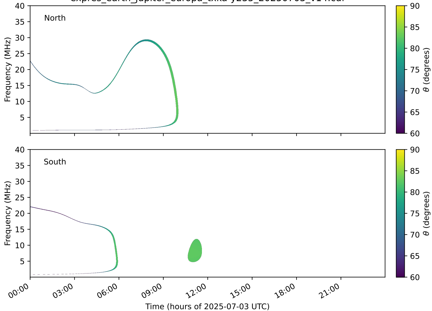
expres_earth_jupiter_europa_txka-y235_20250703_v14.cdf
