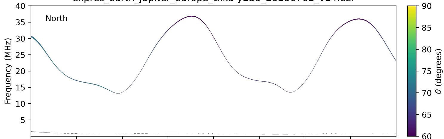
expres_earth_jupiter_europa_txka-y235_20250702_v14.cdf
