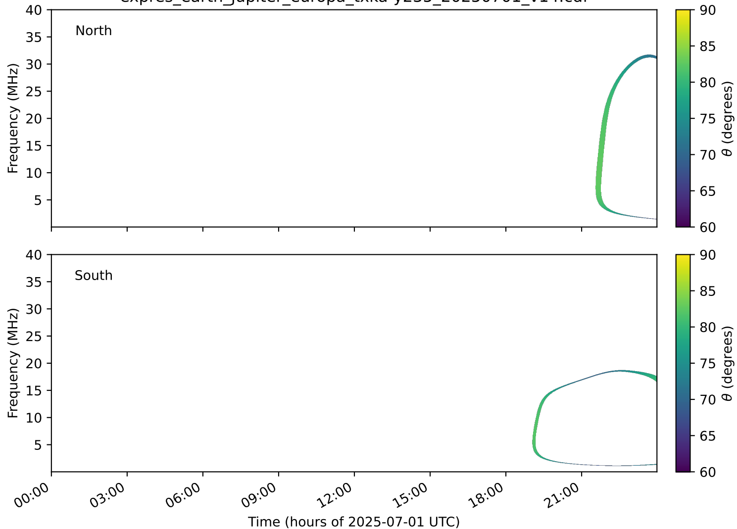
expres_earth_jupiter_europa_txka-y235_20250701_v14.cdf
