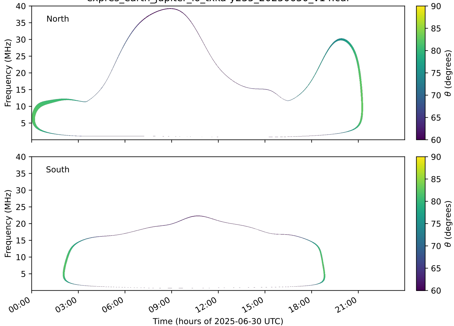
expres_earth_jupiter_io_txka-y235_20250630_v14.cdf
