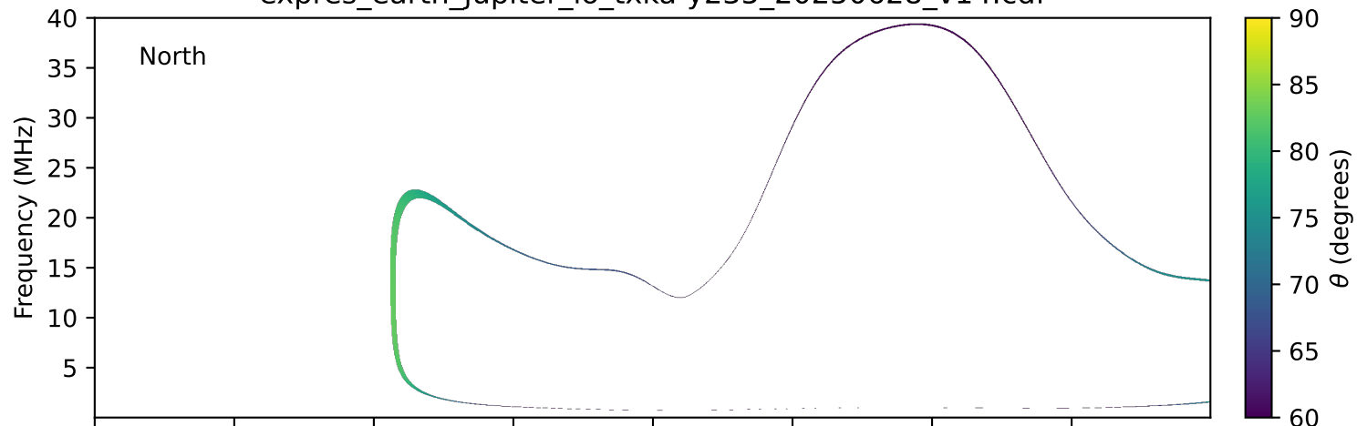
expres_earth_jupiter_io_txka-y235_20250628_v14.cdf
