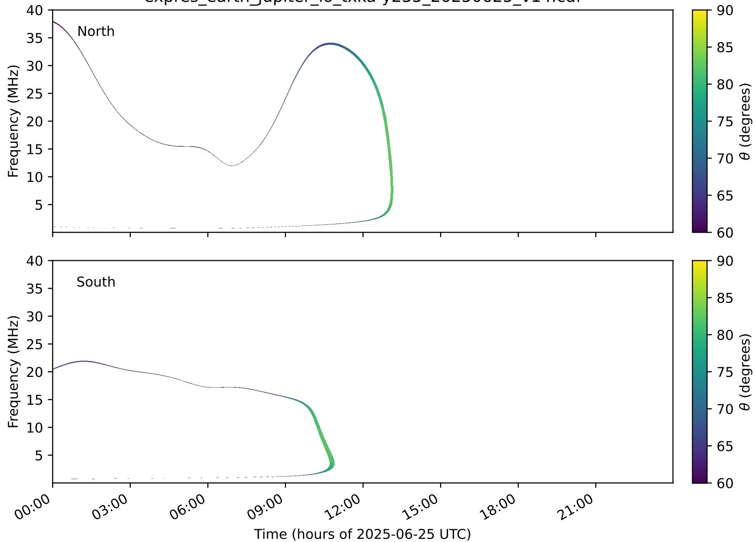
expres_earth_jupiter_io_txka-y235_20250625_v14.cdf
