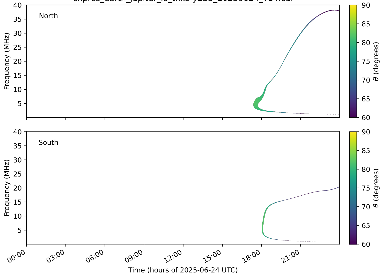
expres_earth_jupiter_io_txka-y235_20250624_v14.cdf
