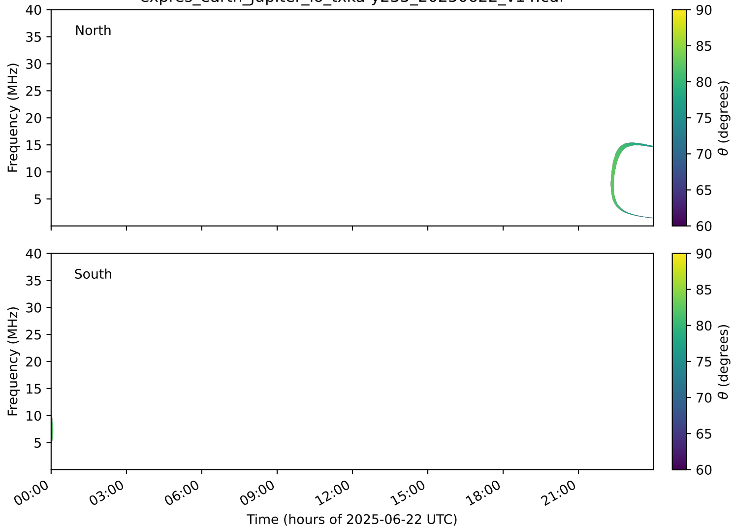
expres_earth_jupiter_io_txka-y235_20250622_v14.cdf
