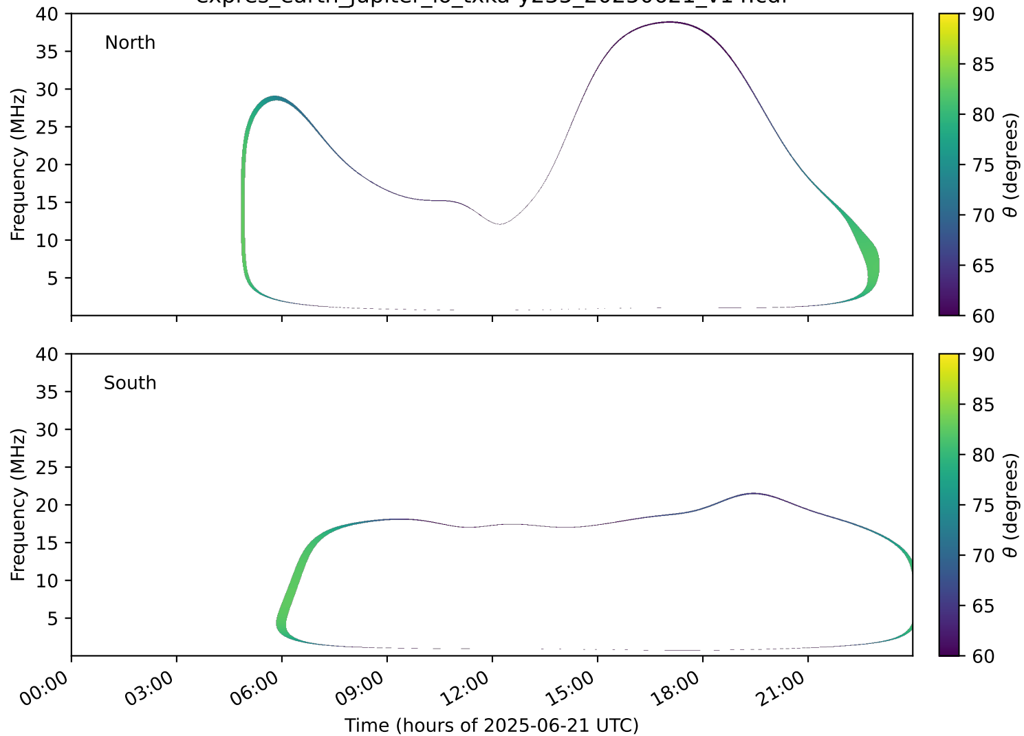
expres_earth_jupiter_io_txka-y235_20250621_v14.cdf
