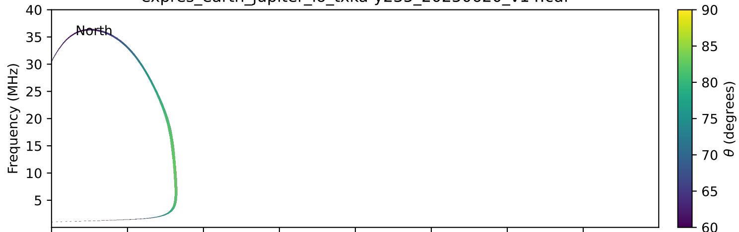
expres_earth_jupiter_io_txka-y235_20250620_v14.cdf
