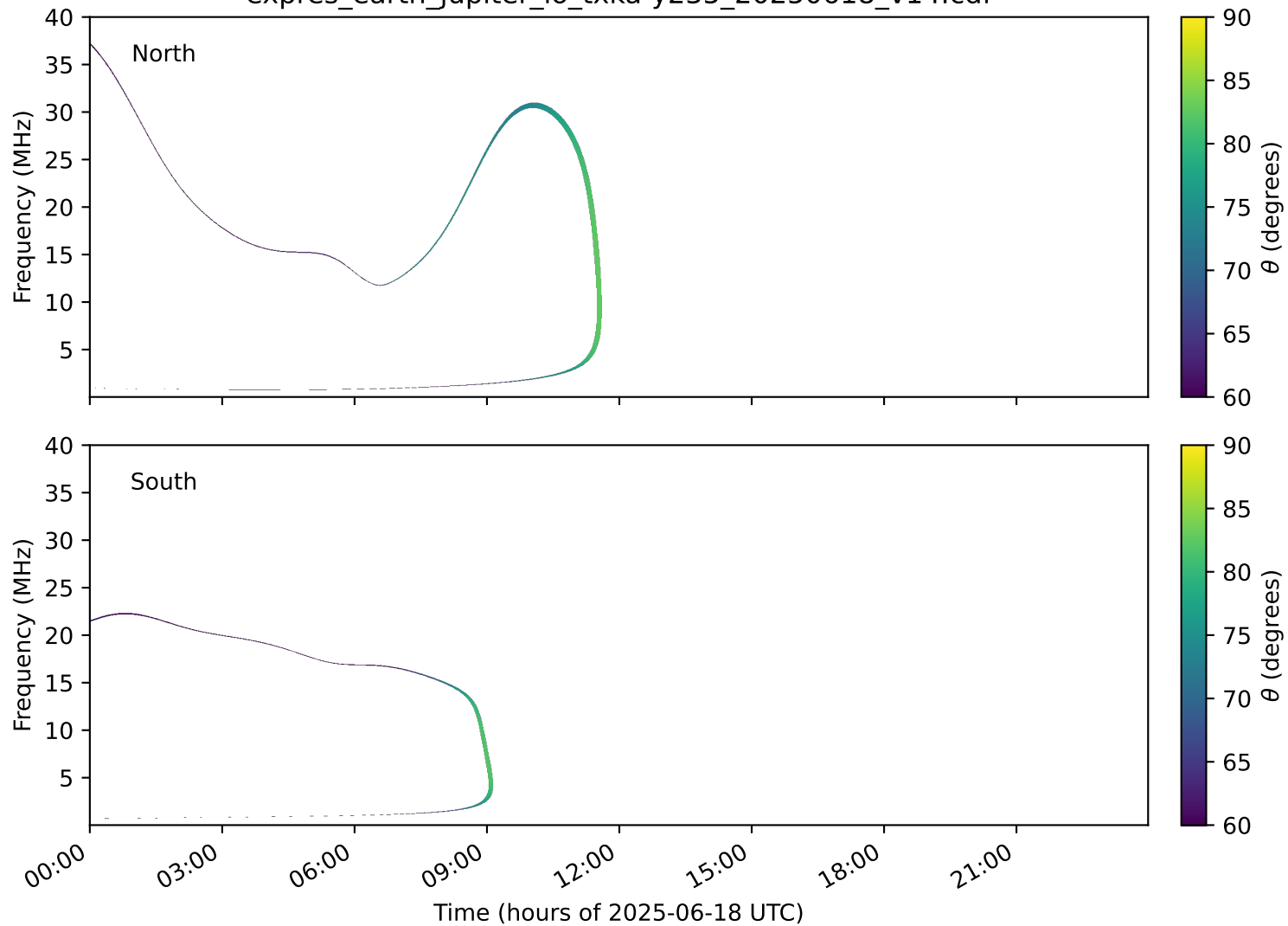
expres_earth_jupiter_io_txka-y235_20250618_v14.cdf
