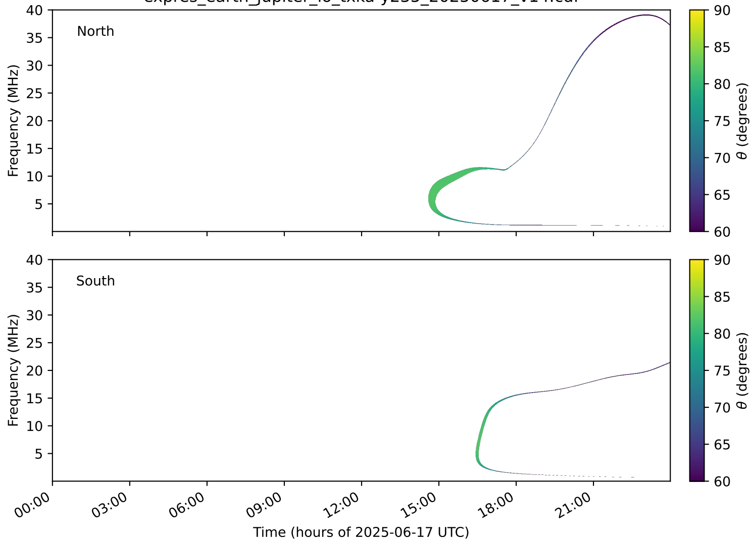
expres_earth_jupiter_io_txka-y235_20250617_v14.cdf
