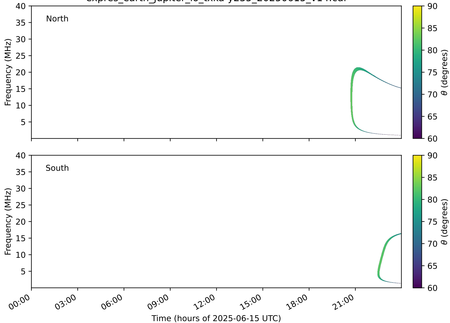
expres_earth_jupiter_io_txka-y235_20250615_v14.cdf
