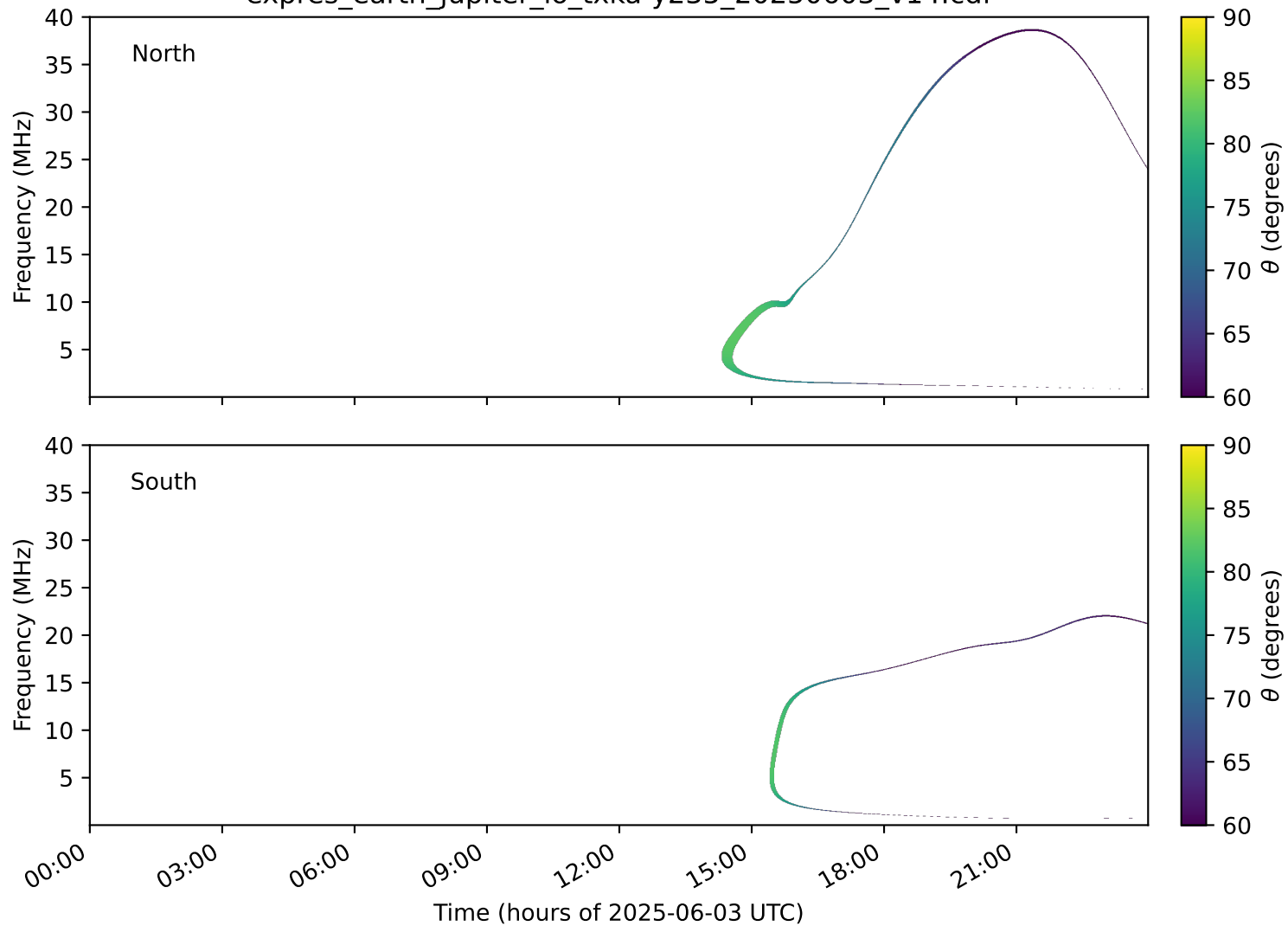
expres_earth_jupiter_io_txka-y235_20250603_v14.cdf
