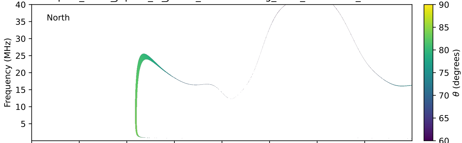
expres_earth_jupiter_io_jrm33_lossc-wid1deg_3kev_20250628_v11.cdf
