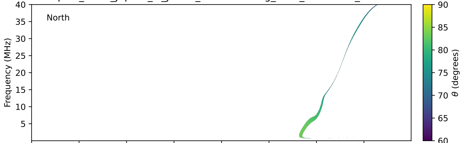
expres_earth_jupiter_io_jrm33_lossc-wid1deg_3kev_20250624_v11.cdf
