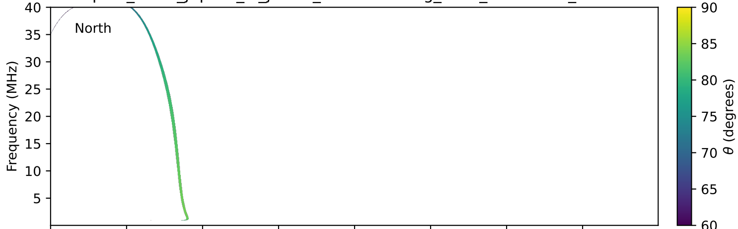
expres_earth_jupiter_io_jrm33_lossc-wid1deg_3kev_20250620_v11.cdf
