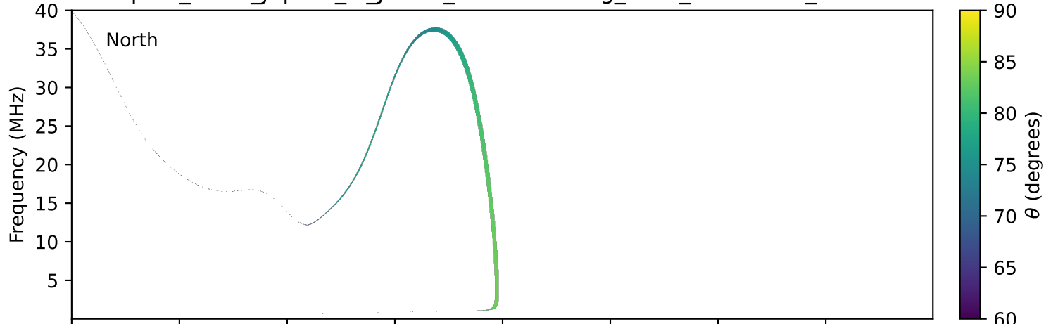
expres_earth_jupiter_io_jrm33_lossc-wid1deg_3kev_20250618_v11.cdf
