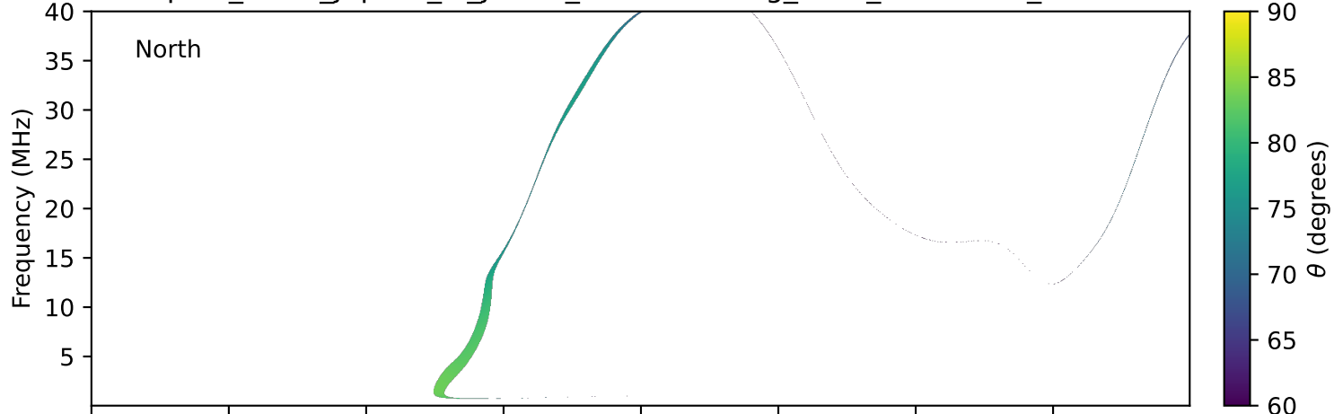
expres_earth_jupiter_io_jrm33_lossc-wid1deg_3kev_20250612_v11.cdf
