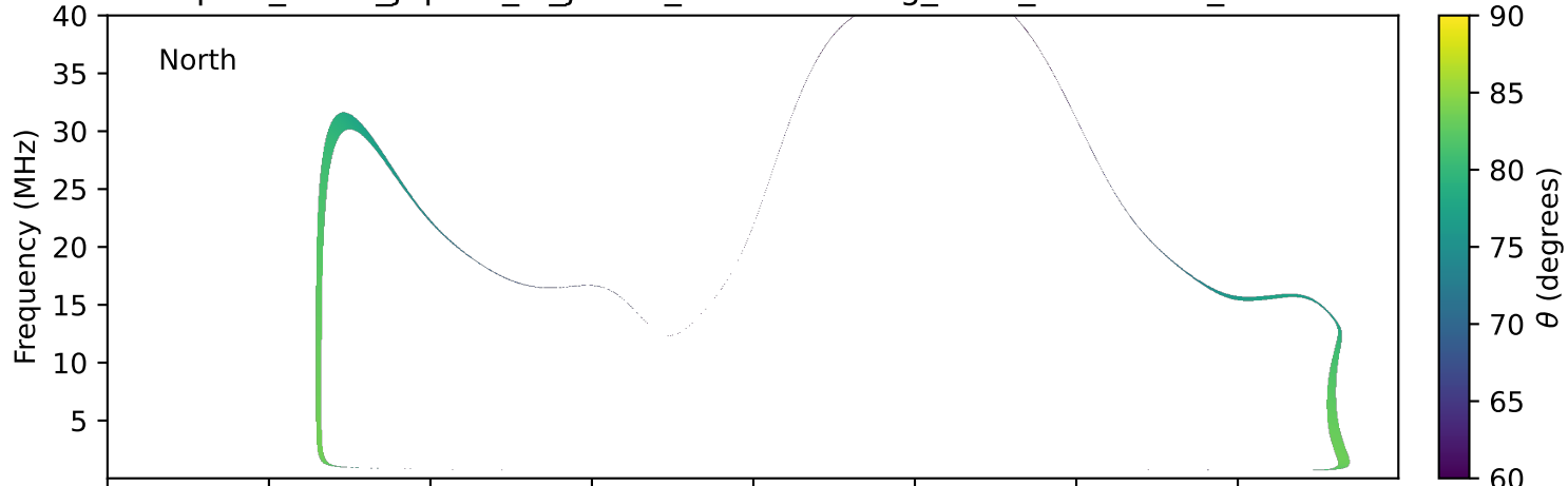
expres_earth_jupiter_io_jrm33_lossc-wid1deg_3kev_20250607_v11.cdf
