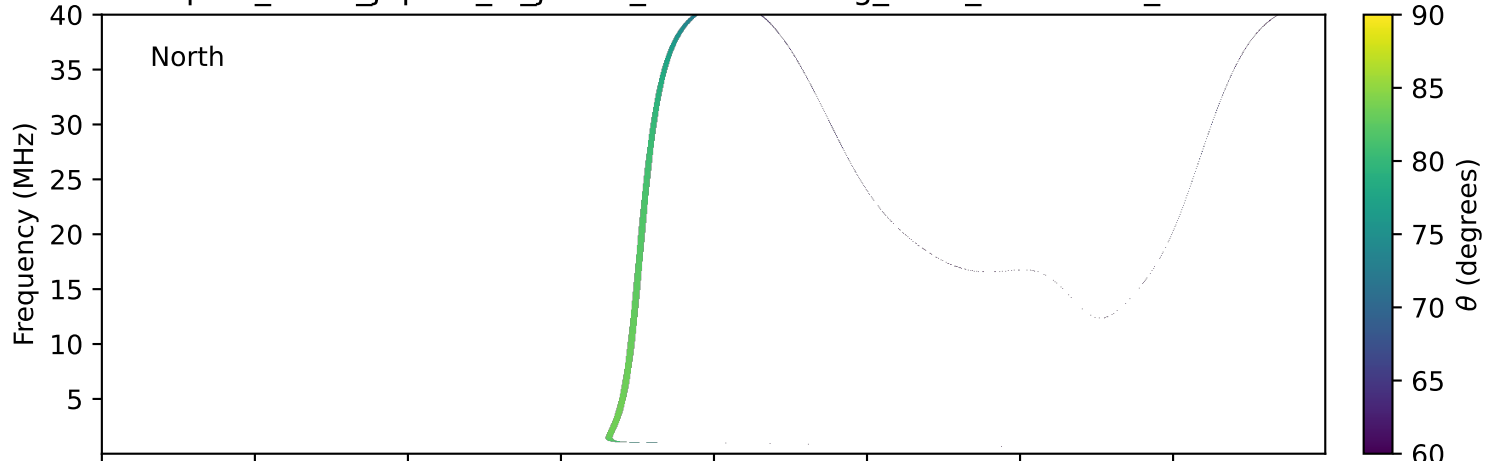
expres_earth_jupiter_io_jrm33_lossc-wid1deg_3kev_20250605_v11.cdf
