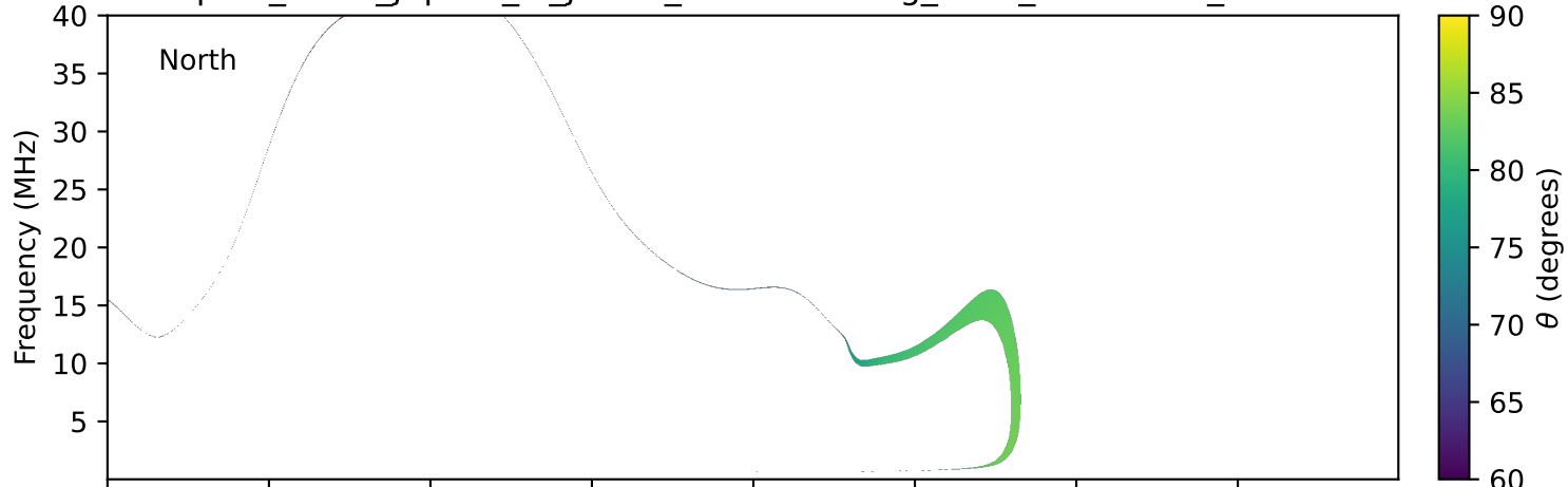
expres_earth_jupiter_io_jrm33_lossc-wid1deg_3kev_20250602_v11.cdf
