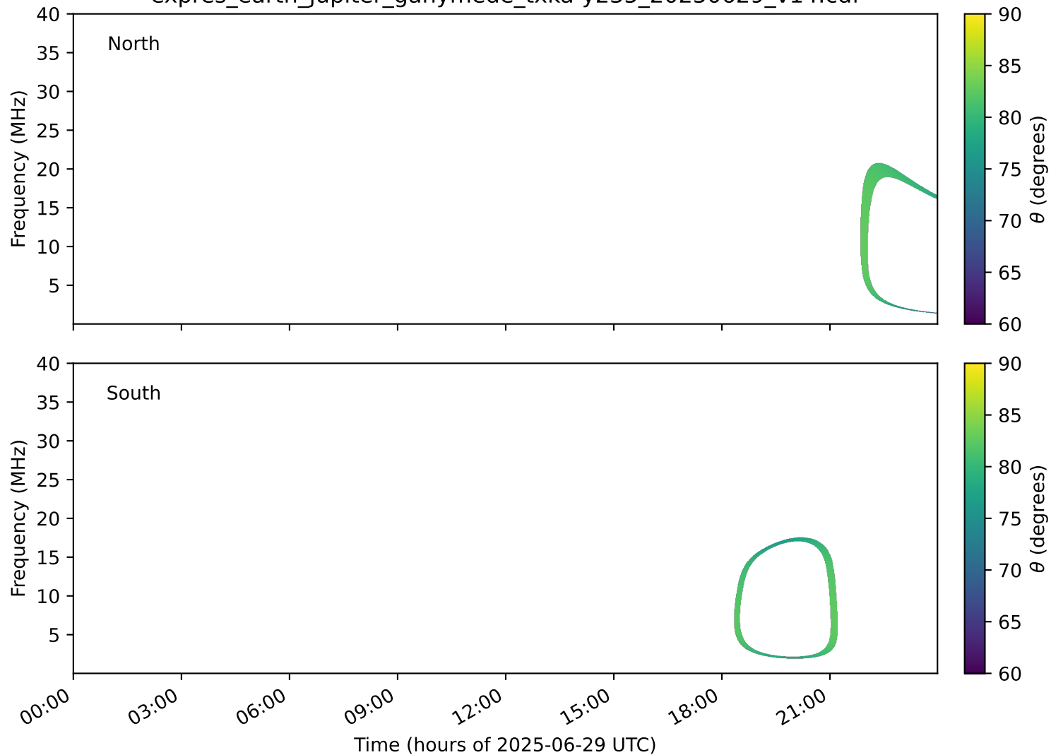
expres_earth_jupiter_ganymede_txka-y235_20250629_v14.cdf
