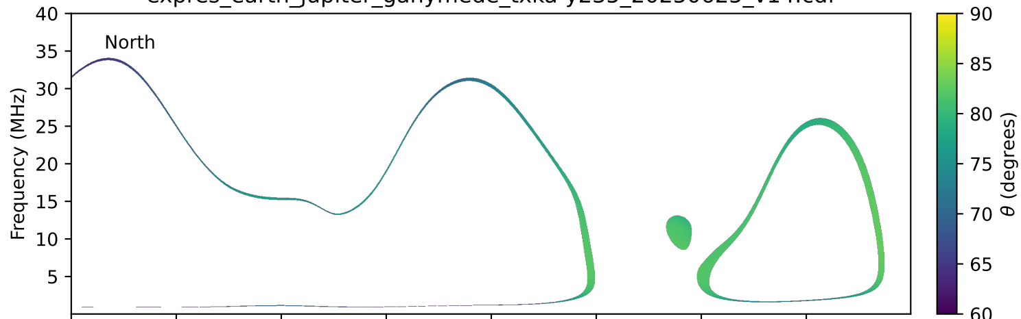
expres_earth_jupiter_ganymede_txka-y235_20250625_v14.cdf
