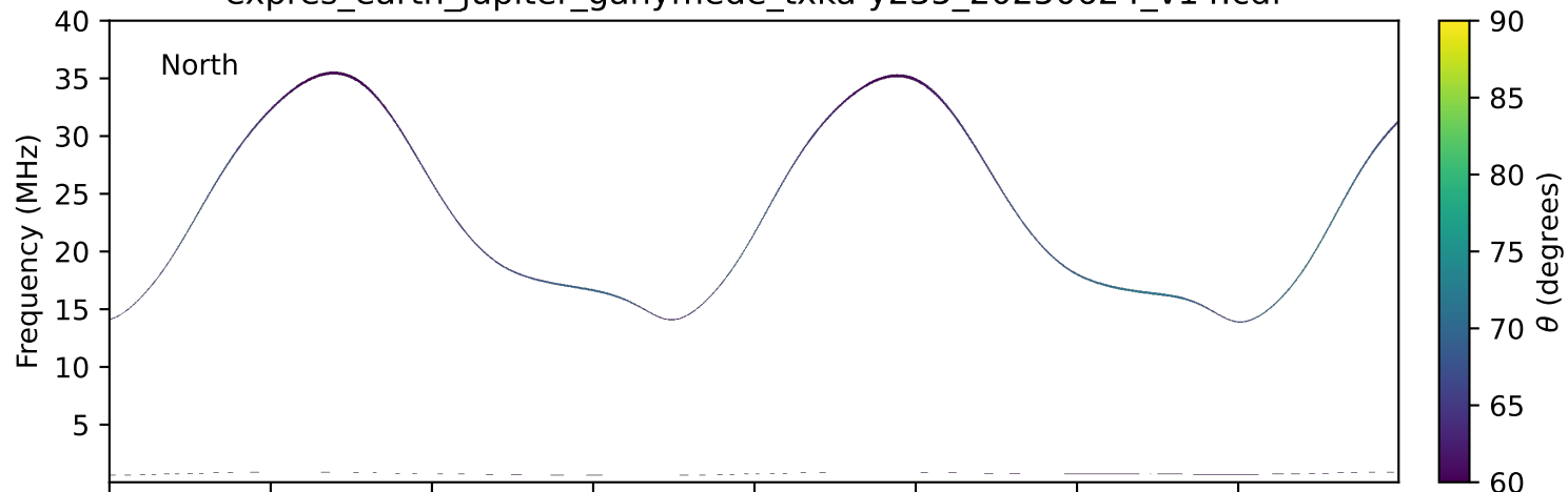
expres_earth_jupiter_ganymede_txka-y235_20250624_v14.cdf
