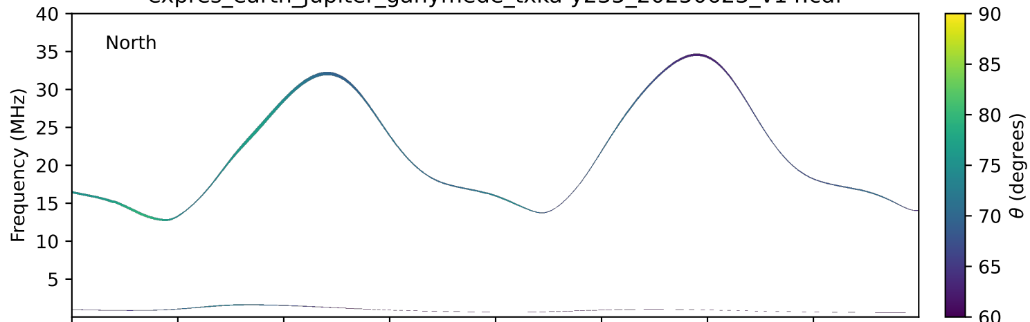
expres_earth_jupiter_ganymede_txka-y235_20250623_v14.cdf
