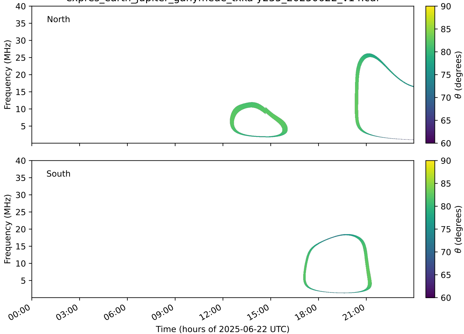
expres_earth_jupiter_ganymede_txka-y235_20250622_v14.cdf
