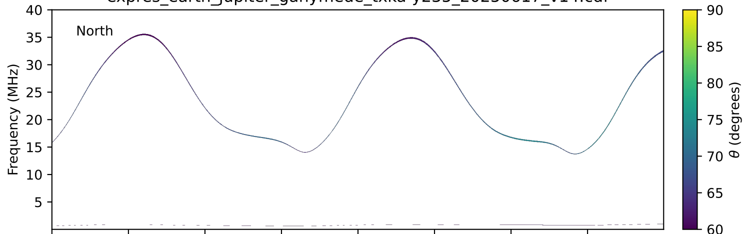
expres_earth_jupiter_ganymede_txka-y235_20250617_v14.cdf
