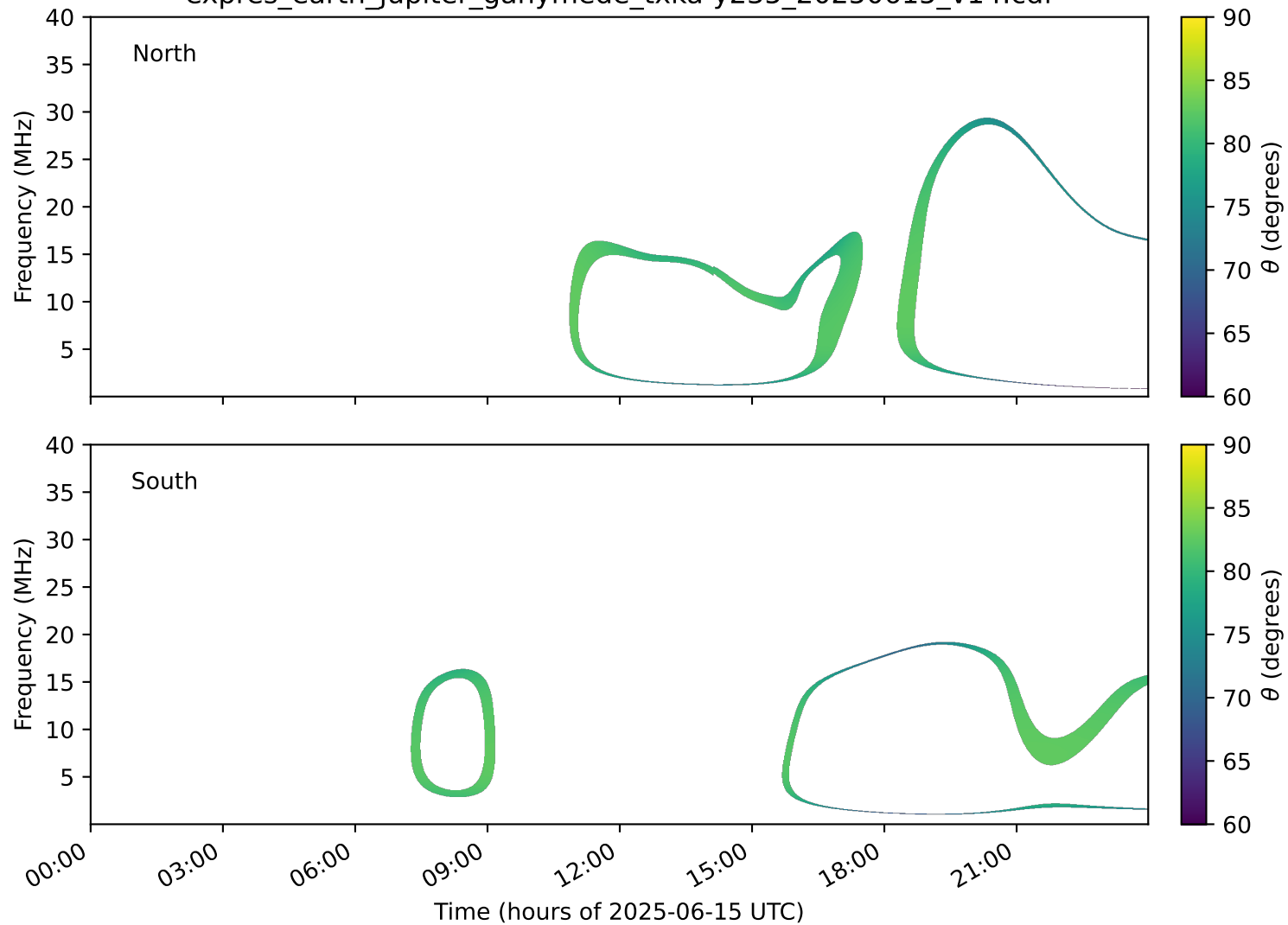
expres_earth_jupiter_ganymede_txka-y235_20250615_v14.cdf
