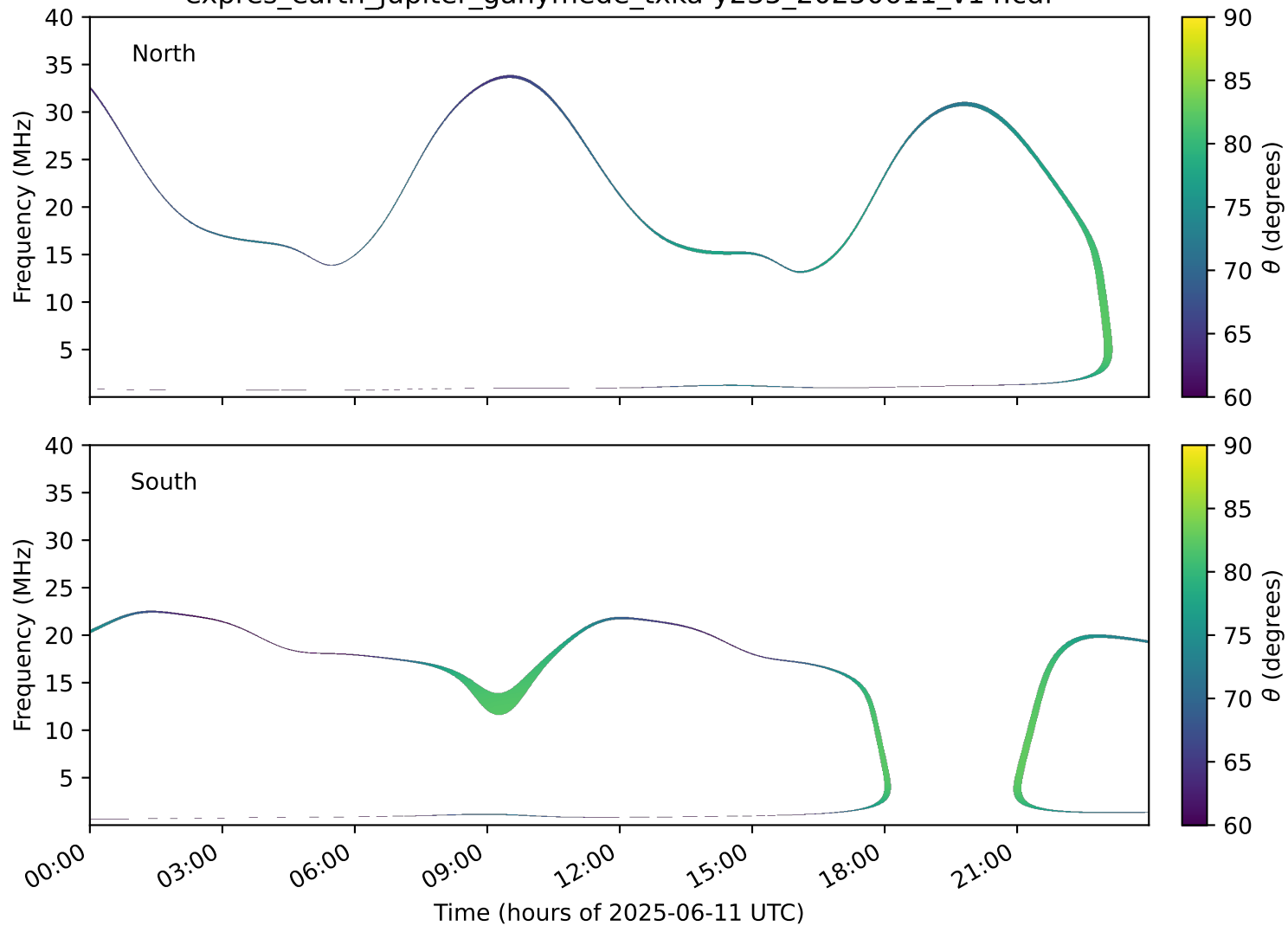
expres_earth_jupiter_ganymede_txka-y235_20250611_v14.cdf
