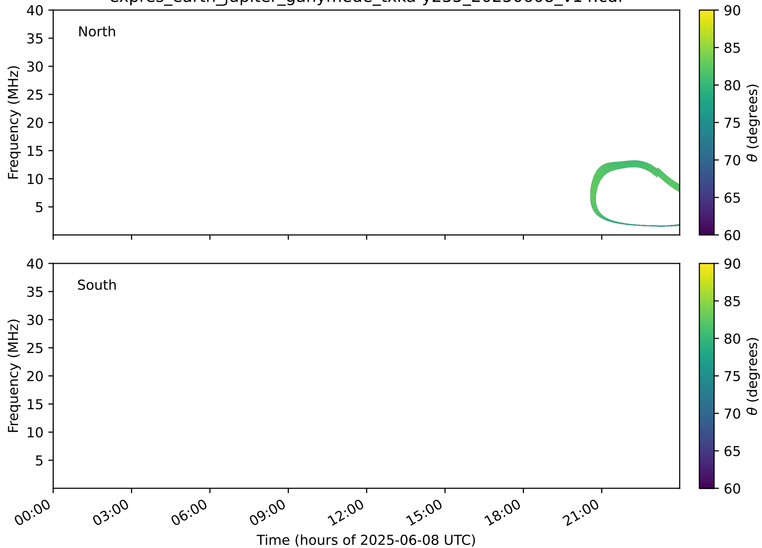
expres_earth_jupiter_ganymede_txka-y235_20250608_v14.cdf
