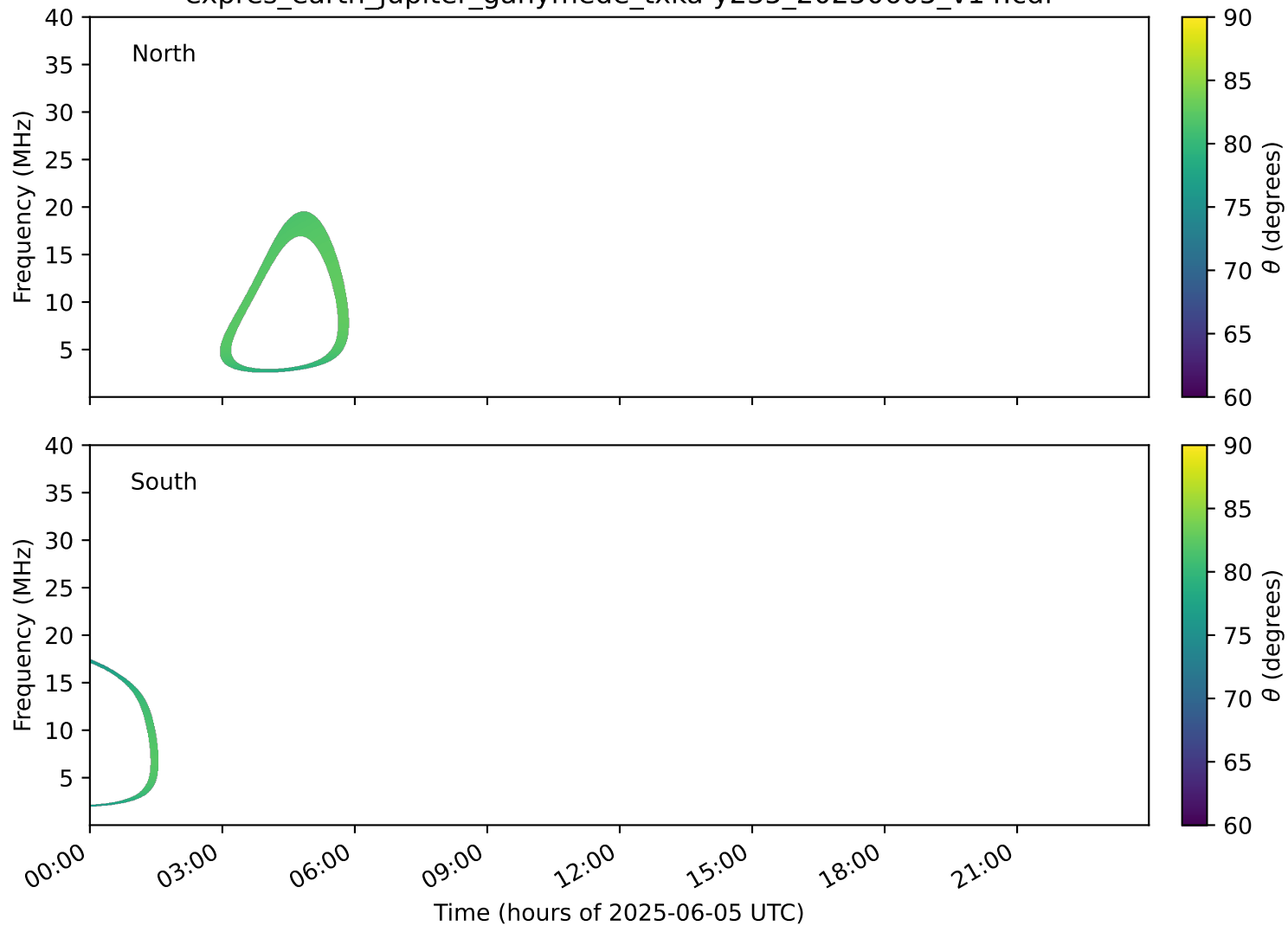
expres_earth_jupiter_ganymede_txka-y235_20250605_v14.cdf
